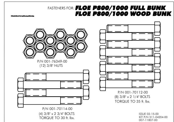
(1) FASTENER KIT - P800/1300 FULL BUNK
